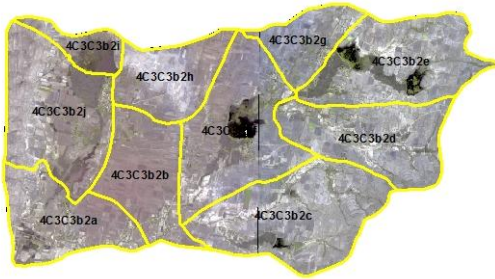
Natural Color Composite- 2011-12
