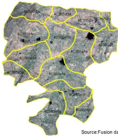
Natural Color Composite- 2011-12
