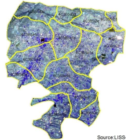
Natural Color Composite- 29th February 2020
