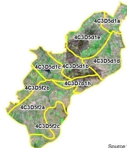
Natural Color Composite - 5th January 2017
