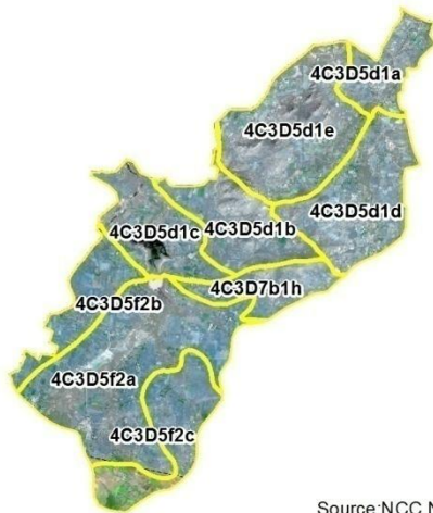
Natural Color Composite - 9th December 2017
