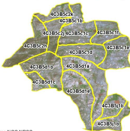
Natural Color Composite - 2nd February 2016
