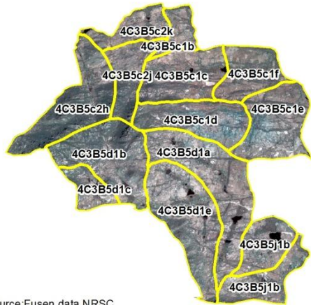
Natural Color Composite - 2011-12
