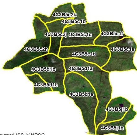
Natural Color Composite - 30th March 2018
