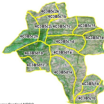
Natural Color Composite - 24th January 2019
