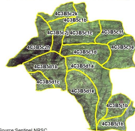
Natural Color Composite - 24th January 2017
