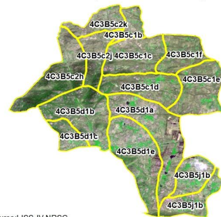
Natural Color Composite - 29th February 2020
