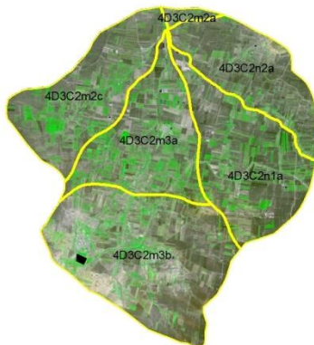
Natural Color Composite-1st April 2018
