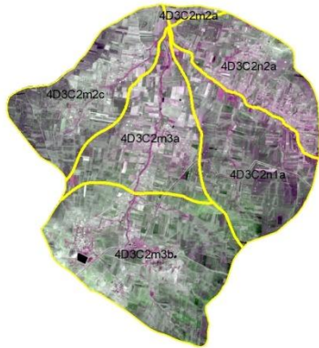
Natural Color Composite- 2011
