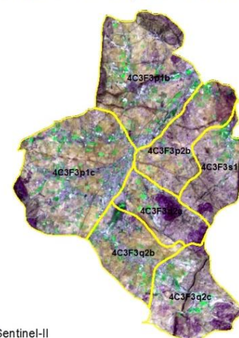
Natural Color Composite- 25th March 2019
