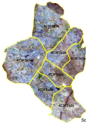
Natural Color Composite- 19th May 2014
