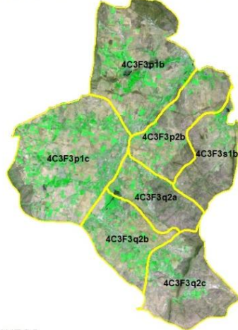
Natural Color Composite- 25th March 2018
