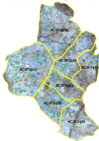
Natural Color Composite- 03 June 2017
